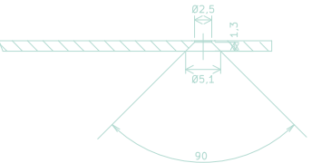
Front panel countersunk hole detail
